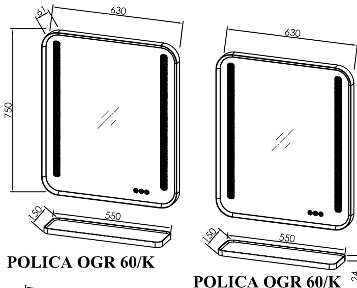
OGR 60 ANT - LED, T, DIF,CCT
